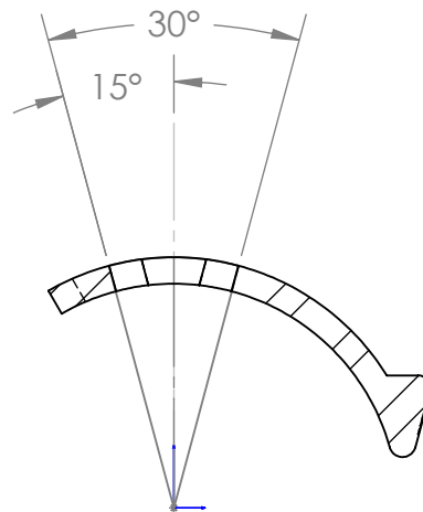
SECTION E-E
